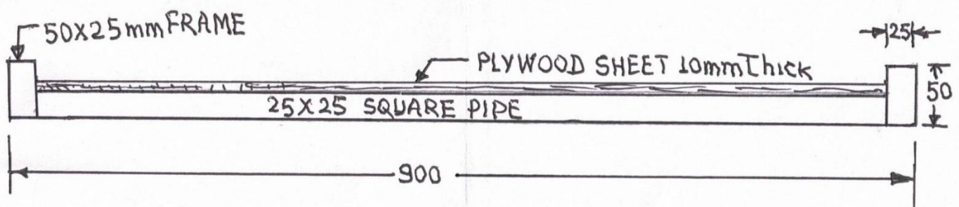
CROSS - SECTION OF BUNK-BED
